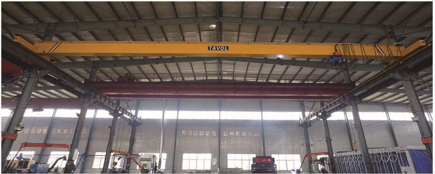
普通方箱单梁桥式起重机 Box type Universal Single Girder Overhead Crane
